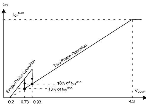
Figure 29. V_{COMP} vs. t_{ON}^{MAX}
