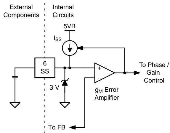
Figure 19. Soft-Start Programming
