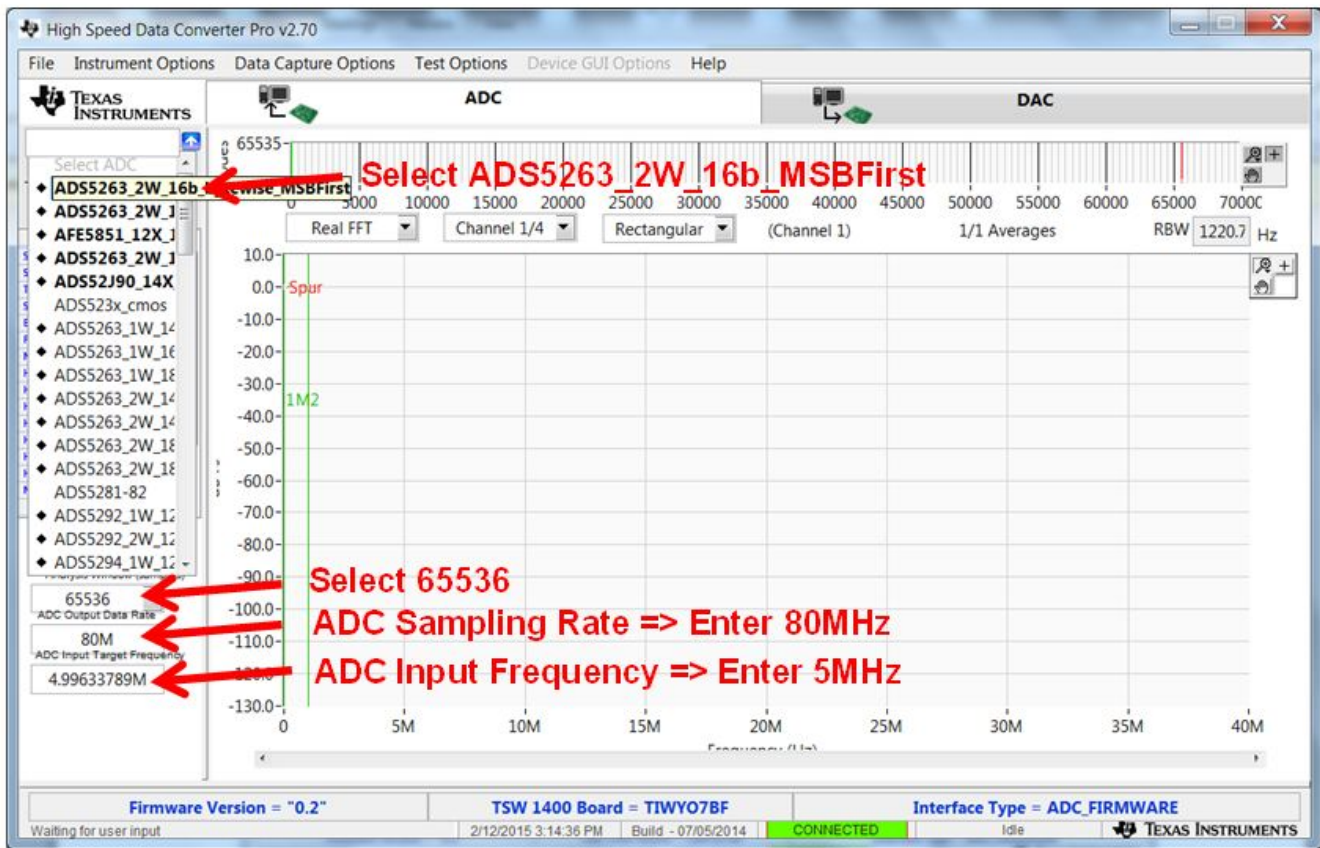
Figure 11. Successful Interface Between TSW Card and Computer
