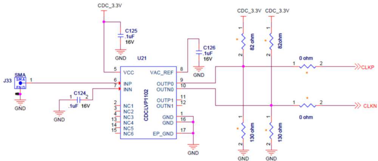
Figure 3. ADS5263 Clocking Using a LVPECL Buffer
