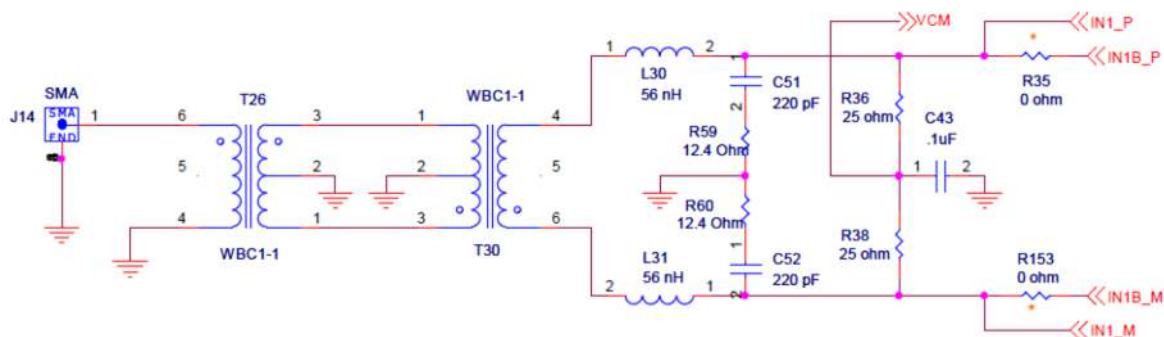
Figure 4. Input Drive Circuit – Using Transformers
