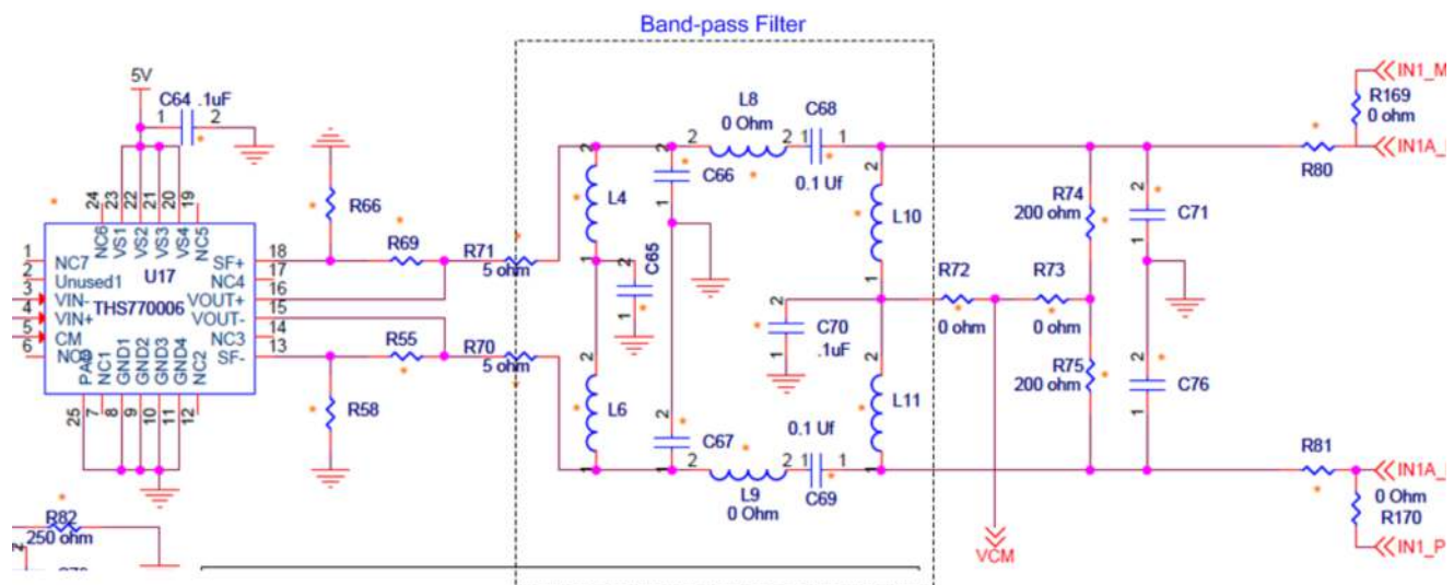
Figure 6. Band-Pass Filter
