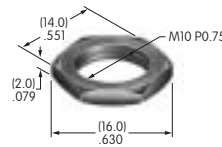
AT530 Panel Mount for Single Pole Polycarbonate Colors: A B C E F G H Series: A AB
