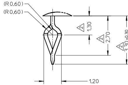
DETAIL1
