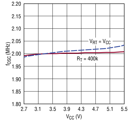
Oscillator Frequency vs V_{\text{CC}}
