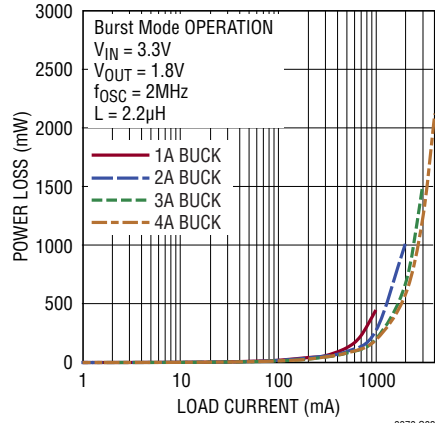
Buck Power Loss vs I_{\text{LOAD}}
