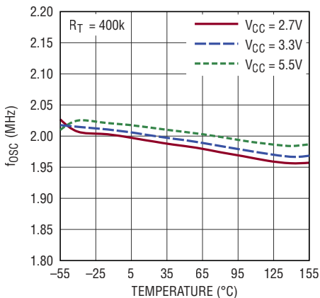
R_{\text{T}} Programmed Oscillator Frequency vs Temperature
