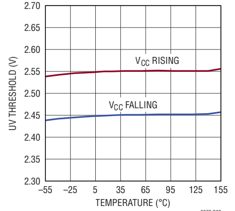
V_{\text{CC}} Undervoltage Threshold vs Temperature
