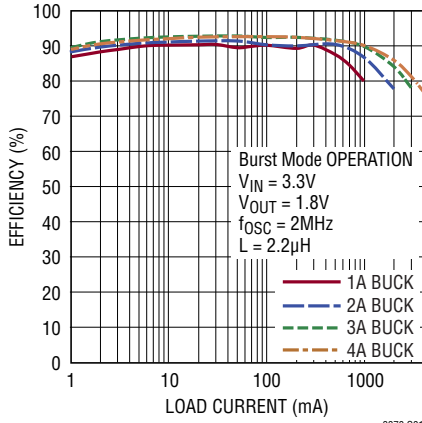
Buck Efficiency vs I_{\text{LOAD}}
