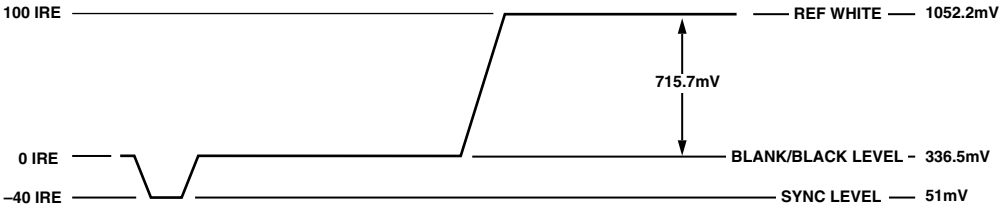
Figure 56. NTSC RGB Video Levels
