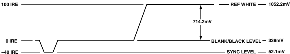
Figure 54. NTSC Luma Video Levels
