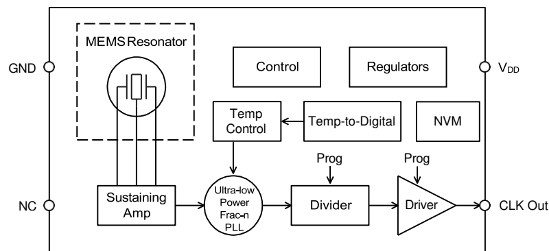
Figure 2. SiT1579 Block Diagram
