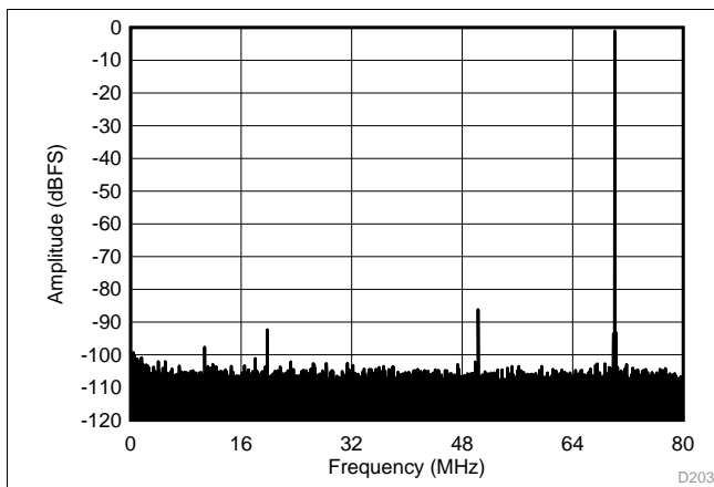
Figure 154. FFT with Dither On
