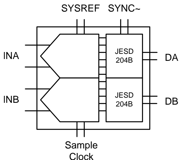
Figure 156. JESD204B Interface
