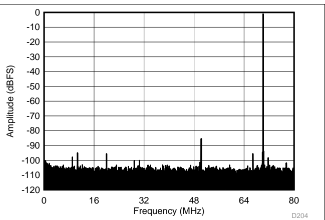
Figure 155. FFT with Dither Off
