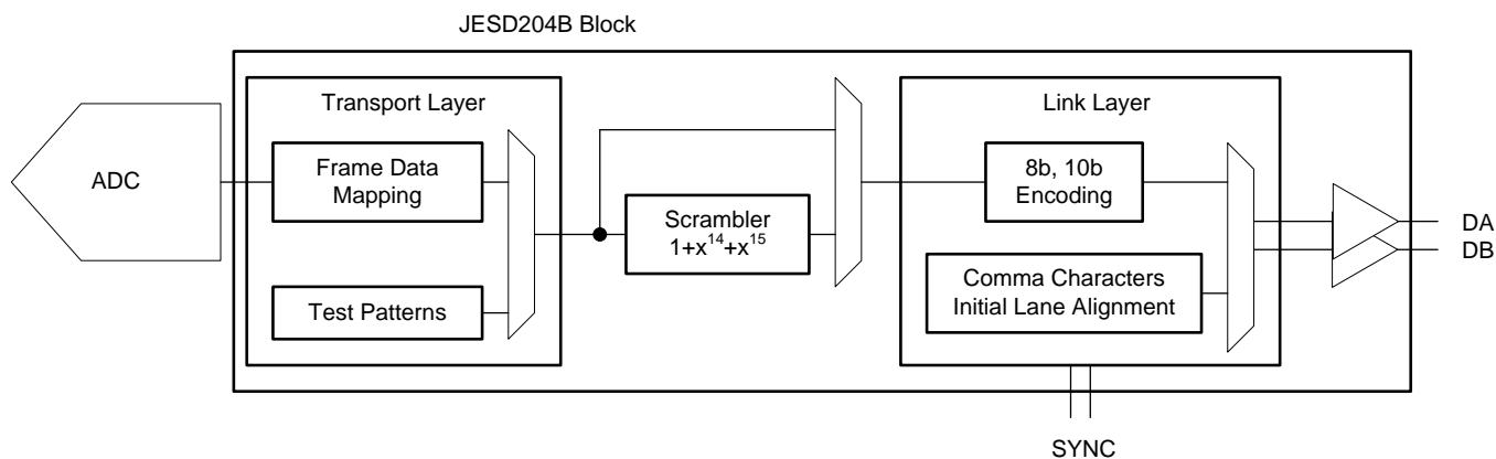
Figure 157. JESD204B Block
