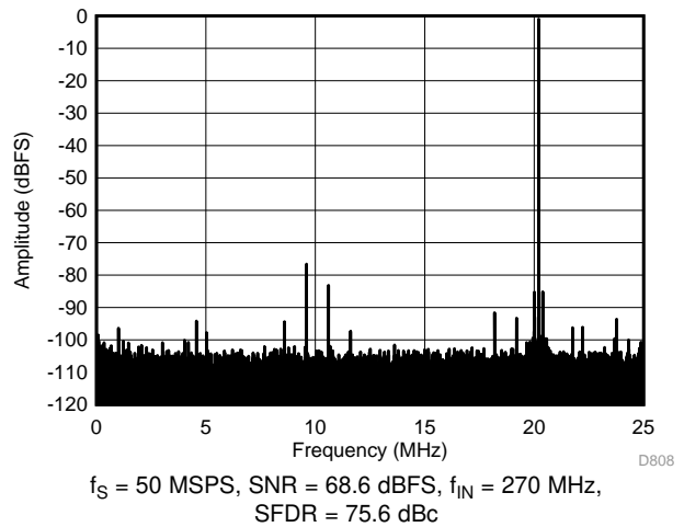
Figure 107. FFT for 270-MHz Input Signal (Dither Off)
