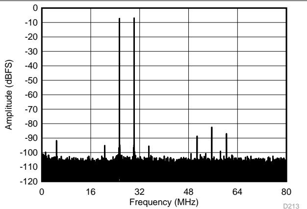
f_S = 160\text{ MSPS} , \text{IMD} = 82.5\text{ dBFS} , f_{IN1} = 185\text{ MHz} , f_{IN2} = 190\text{ MHz}
