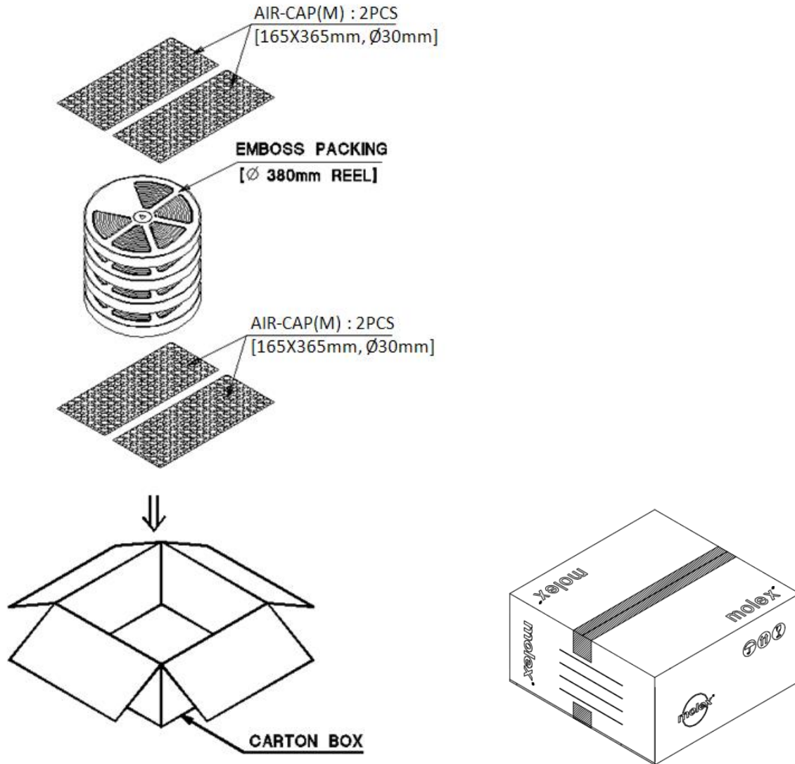
[ Packing Process ]
