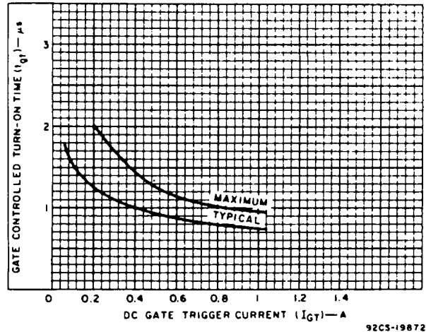
Fig.12—Gate-controlled turn-on time vs. gate trigger current.
