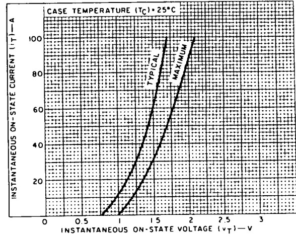
Fig. 6—Instantaneous on-state current vs. on-state voltage.
