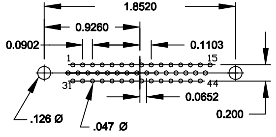
44 POSITION MALE
