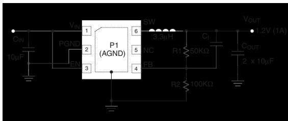
Figure 4. Setting the Output Voltage
