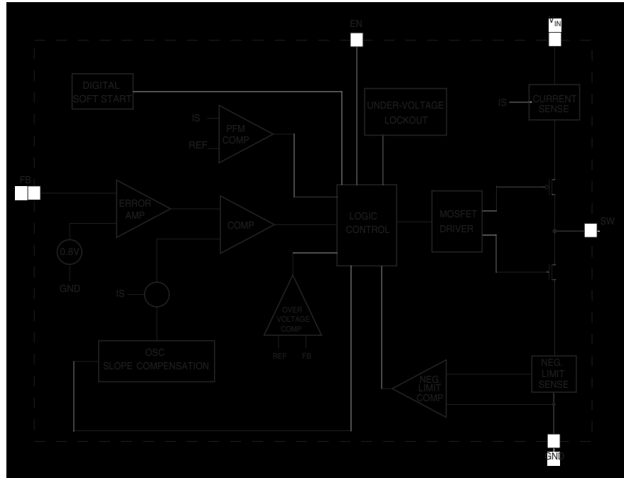
Figure 3. Block Diagram
