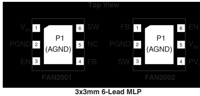
Figure 2. Pin Assignment
