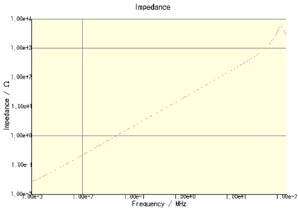
CLF6045T-3R3N-CA
