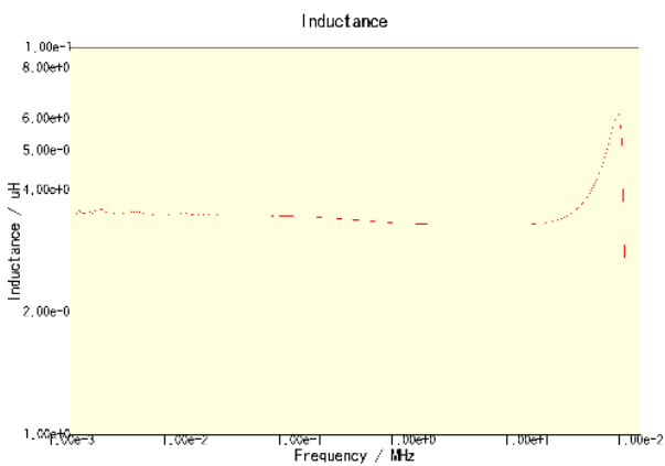
CLF6045T-3R3N-CA
