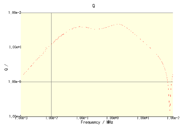
CLF6045T-3R3N-CA
