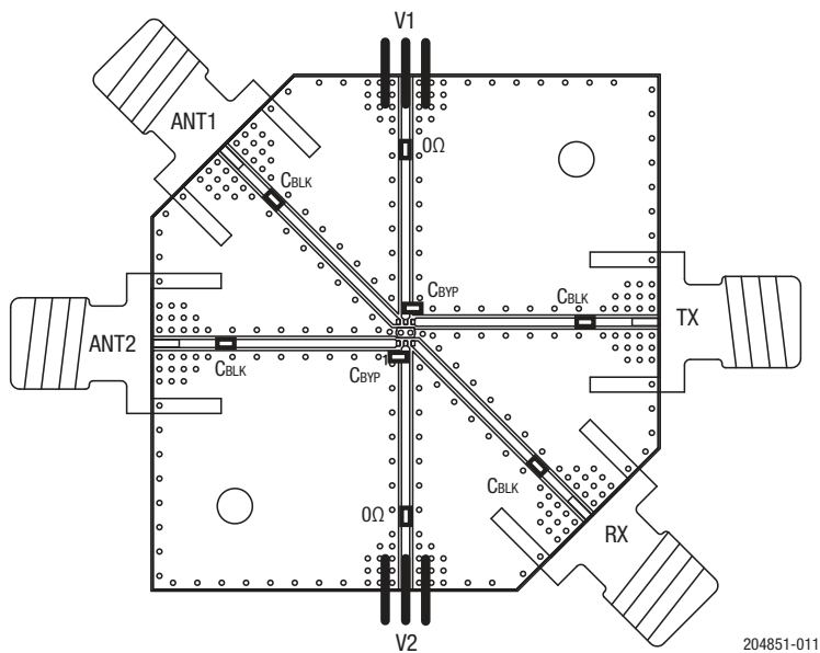
Figure 11. SKYA21070 Evaluation Board Assembly Diagram
