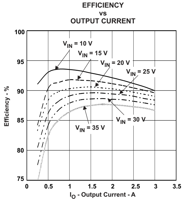
Figure 2-1. TPS5430 Efficiency
