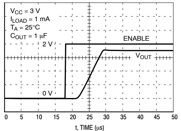
Figure 21. Enable Response
