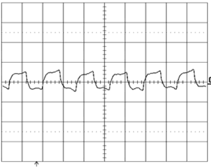
Output voltage ripple (20mV/div.) at: T_{ref} = +25^{\circ}C , I_O = 30 A resistive load, V_i = 3.3 V. Time scale: 2 \mu s/div. See the filter in the Output ripple and noise section (EMC Specification).
