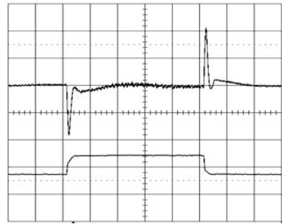
Output voltage response to load current step- change (15-30-15 A) at: T_{ref} = +25^{\circ}C , V_i = 3.3 V. Top trace: output voltage (100mV/div.). Bottom trace: load current (20 A/div.). Time scale: 0.1 ms/div..
