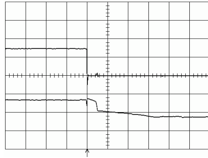
Shut-down enabled by disconnecting V_i at: T_{ref} = +25^{\circ}C , I_O = 30 A resistive load, V_i = 3.3 V. Top trace: output voltage (1.0 V/div.). Bottom trace: input voltage (2 V/div.). Time scale: 5.0 ms/div..
