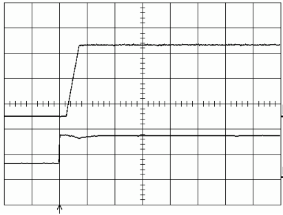
Start-up enabled by connecting V_i at: T_{ref} = +25^{\circ}C , I_O = 30 A resistive load, V_i = 3.3 V. Top trace: output voltage (0.5 V/div.). Bottom trace: input voltage (2 V/div.). Time scale: 10 ms/div..
