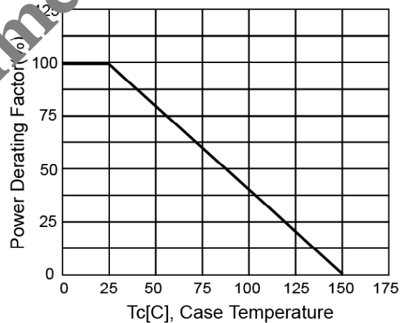
Figure 4. Power Derating
