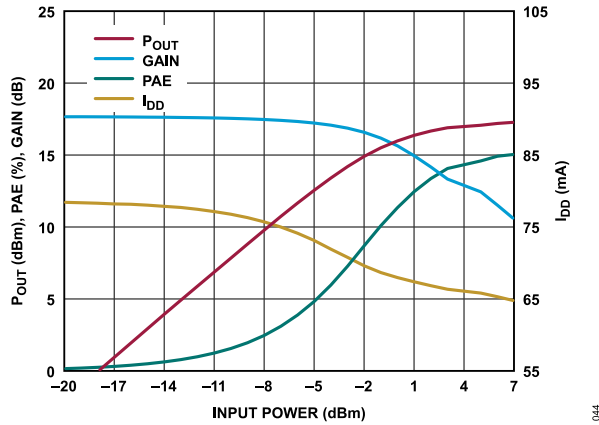
Figure 44. P_{OUT} , PAE, Gain, and I_{DD} vs. Input Power, Power Compression at 1 GHz, V_{DD} = 5\text{ V} , V_{BIAS} = 5\text{ V} , R_{BIAS} = 300\ \Omega
