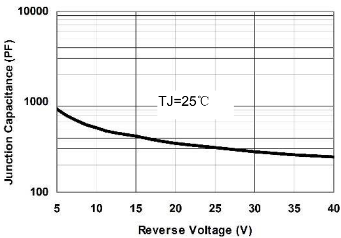
Fig.1-Typical Junction Capacitance
