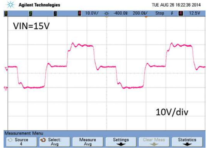
Figure 4. Switch Node Voltage, V_{IN} = 15V
