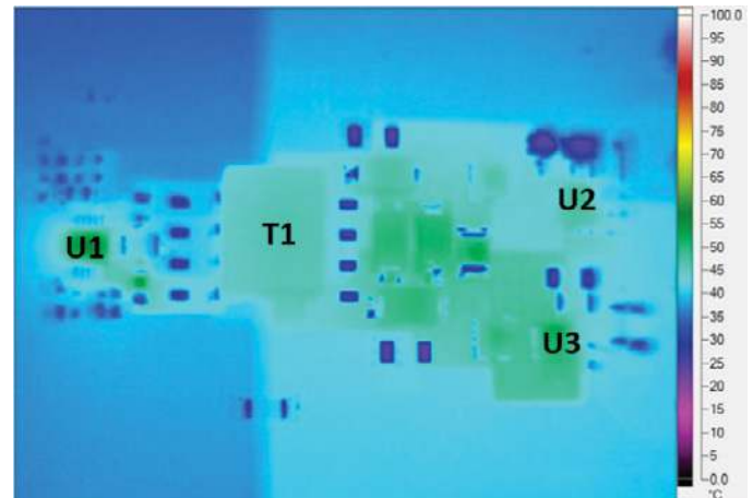
Figure 6. Thermal Image, V_{IN} = 15V , I_{OUT1} = I_{OUT2} = 200mA
