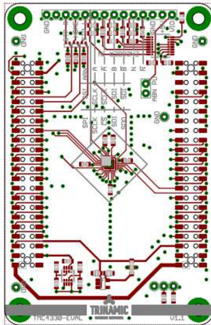
Figure 62: Components Assembly for Application with Encoder
