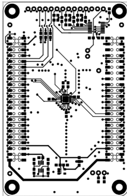
Figure 63: Top Layer: Assembly Side
