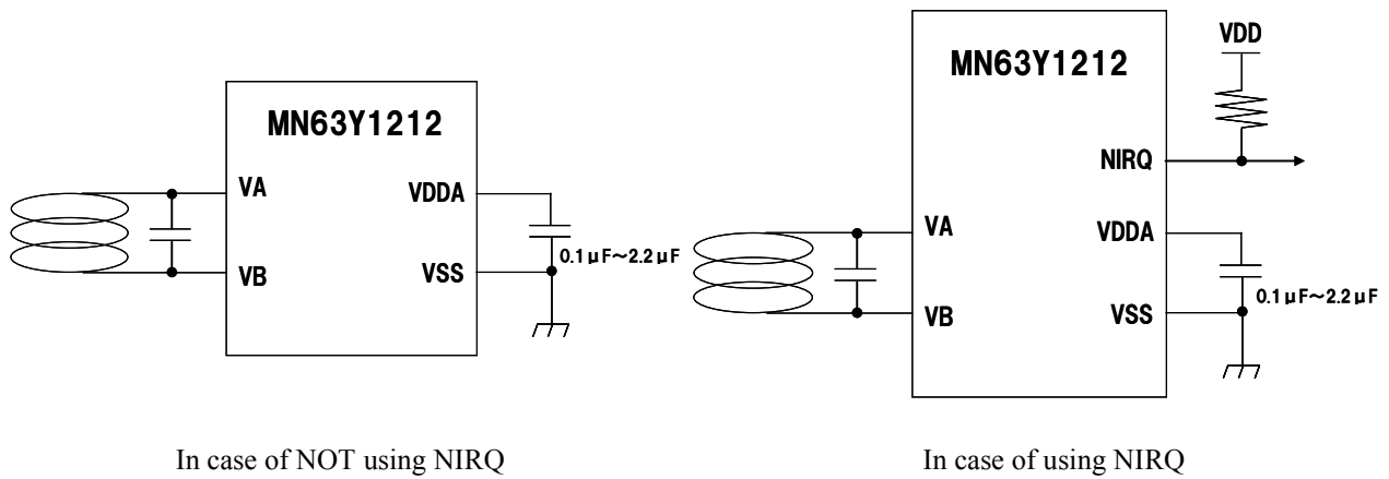
Figure 2-3 Connection Example
