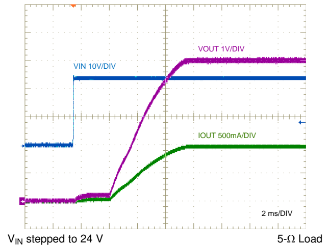
Figure 29. Start-up Characteristic
