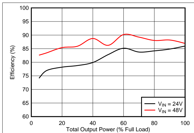
Figure 52. Efficiency
