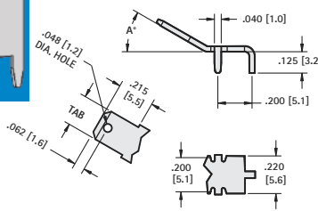
.110 (2.8) & .187 (4.8) TAB
