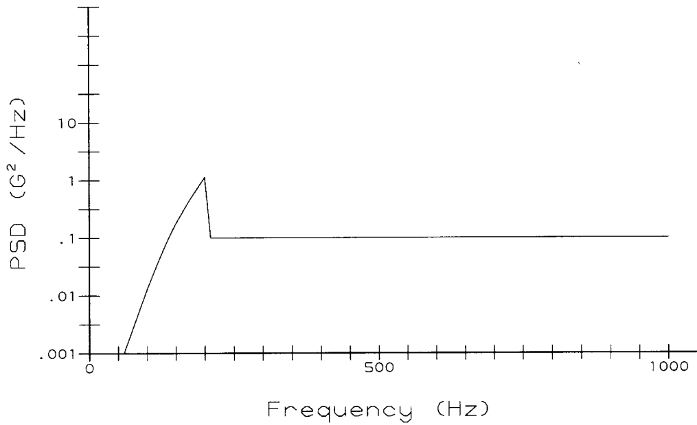
Figure 6 Vibration Profile
