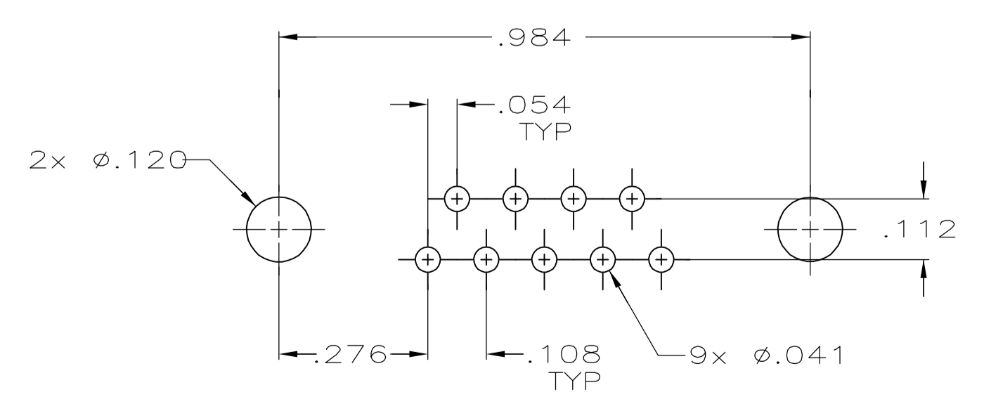
P.C. BOARD MOUNTING DIMENSIONS \Delta
