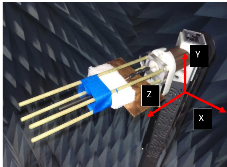
Chamber Setup
