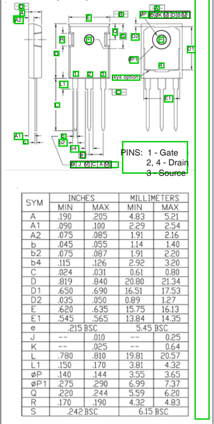
TO-247 (IXTH) Outline
