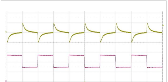
Output voltage response to load current step- change (5.0-7.5-5.0 A) at: T_{P1} = +25^\circ\text{C} , V_I = 110\text{ V} . Top trace: output voltage (500 mV/div.). Bottom trace: load current (2 A/div.). Time scale: (1ms/div.).
