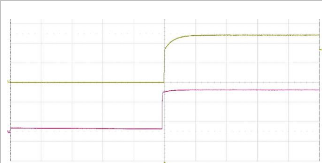
Start-up enabled by connecting V_i at: T_{P1} = +25^\circ\text{C} , V_i = 110\text{ V} , I_o = 6.25\text{ A} resistive load. Top trace: output voltage (10 V/div.). Bottom trace: input voltage (50 V/div.). Time scale: (50 ms/div.).
