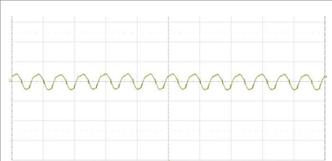
Output voltage ripple at: T_{PI} = +25^{\circ}\text{C} , V_i = 110\text{ V} , I_o = 6.67\text{ A} resistive load. Trace: output voltage (50 mV/div.). Time scale: (5 μs/div.).
