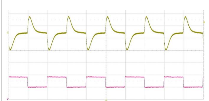
Output voltage response to load current step-change (3.335-5.003-3.335 A) at: T_{PI} = +25^{\circ}\text{C} , V_i = 110\text{ V} . Trace: output voltage (500 mV/div.). Bottom trace: load current (2 A/div.). Time scale: (1ms/div.).
