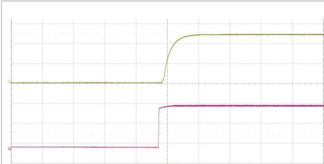
Start-up enabled by connecting V_I at: T_{P1} = +25^\circ\text{C} , V_I = 110\text{ V} , I_O = 12.5\text{ A} resistive load. Top trace: output voltage (5 V/div.). Bottom trace: input voltage (50 V/div.). Time scale: (50 ms/div.).
