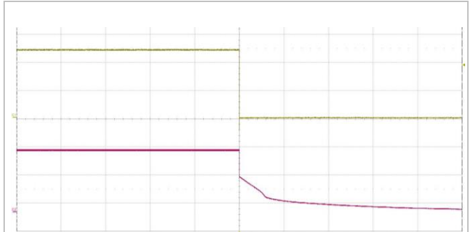
Shut-down enabled by disconnecting V_I at: T_{P1} = +25^\circ\text{C} , V_I = 110\text{ V} , I_O = 12.5\text{ A} resistive load. Top trace: output voltage (5 V/div.). Bottom trace: input voltage (50 V/div.). Time scale: (500 ms/div.).
