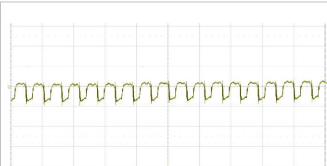
Output voltage ripple at: T_{P1} = +25^\circ\text{C} , V_i = 110\text{ V} , I_o = 6.25\text{ A} resistive load. Trace: output voltage (20 mV/div.). Time scale: (5 μs/div.).
