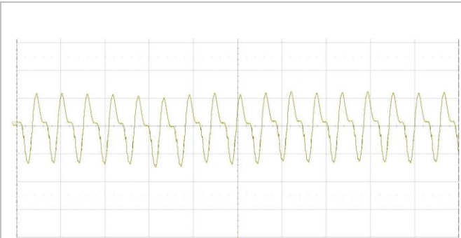
Output voltage ripple at: T_{P1} = +25^{\circ}\text{C} , V_i = 110\text{ V} , I_o = 3.12\text{ A} resistive load. Trace: output voltage (100 mV/div.). Time scale: (5 \mu\text{s} /div.).
