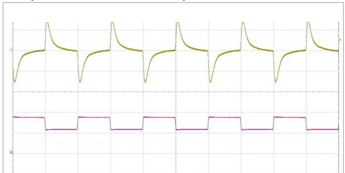
Output voltage response to load current step- change (6.25-9.375-6.25 A) at: T_{P1} = +25^\circ\text{C} , V_I = 110\text{ V} . Top trace: output voltage (500 mV/div.). Bottom trace: load current (5 A/div.). Time scale: (1ms/div.).
