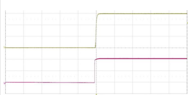
Start-up enabled by connecting V_I at: T_{P1} = +25^\circ\text{C} , V_I = 110\text{ V} , I_O = 10\text{ A} resistive load. Top trace: output voltage (5 V/div.). Bottom trace: input voltage (50 V/div.). Time scale: (100 ms/div.).
