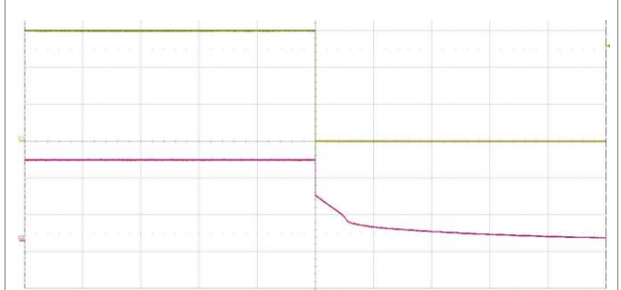
Start-up enabled by connecting V_i at: T_{PI} = +25^{\circ}\text{C} , V_i = 110\text{ V} , I_o = 6.67\text{ A} resistive load. Top trace: output voltage (5 V/div.). Bottom trace: input voltage (50 V/div.). Time scale: (500 ms/div.).
