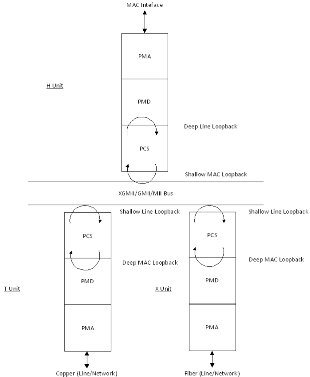
Figure 5: Loopback Paths
