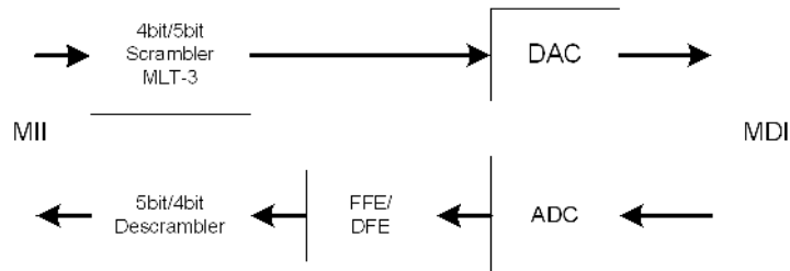
Figure 16: 100BASE-TX Data Path
