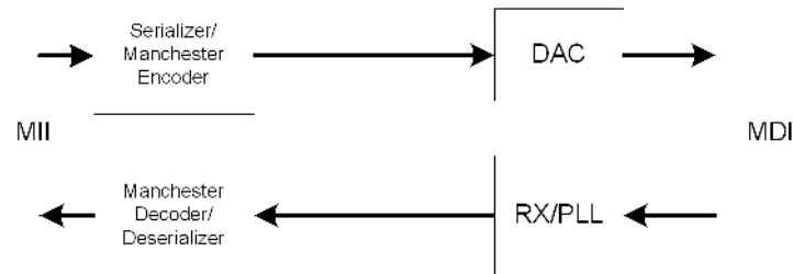
Figure 17: 10BASE-T Data Path
