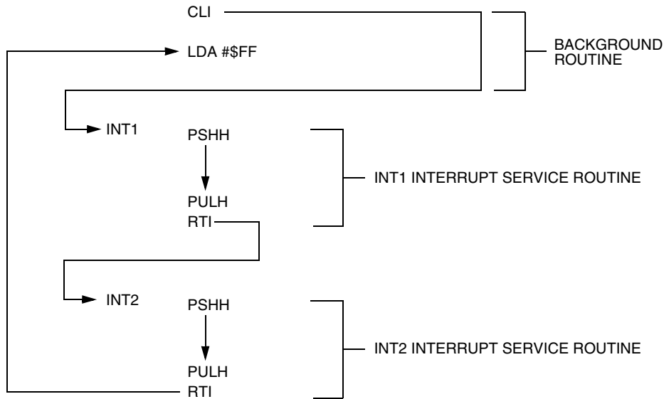
Figure 4-11. Interrupt Recognition Example
