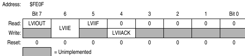
Figure 14-2. LVI Status Register (LVISR)
