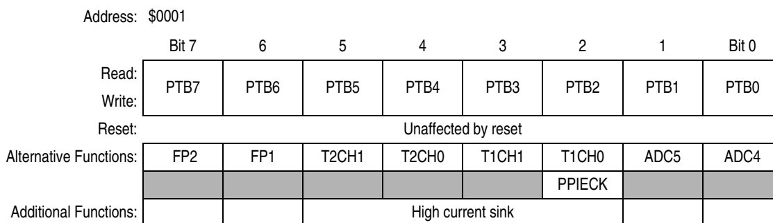
Figure 10-5. Port B Data Register (PTB)
