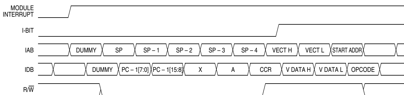
Figure 4-8. Interrupt Entry Timing
