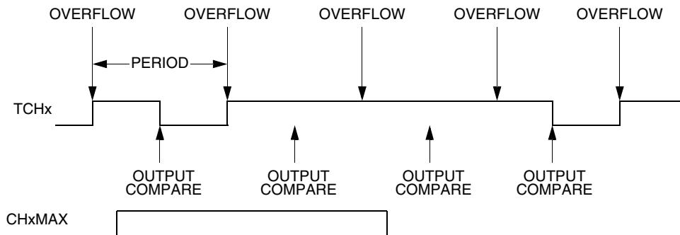
Figure 6-11. CHxMAX Latency
