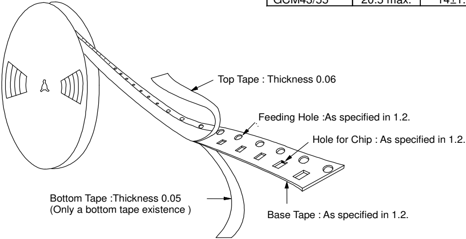
Fig.3 Taping Diagram
