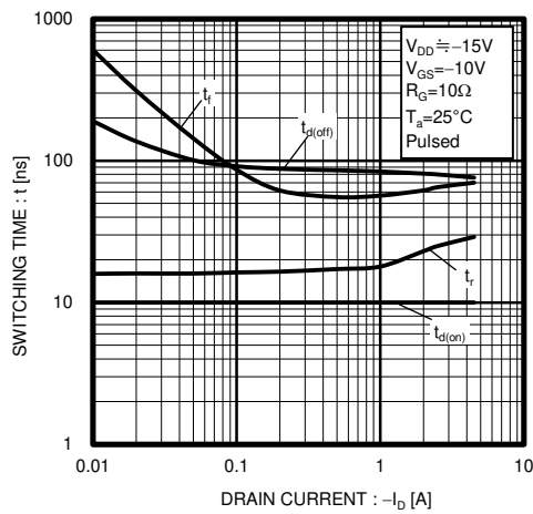
Fig.11 Switching Characteristics
