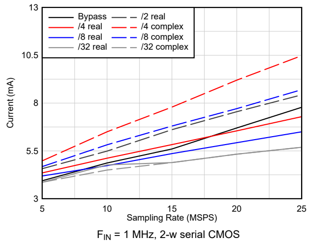
Figure 6-16. I_{OVDD} Current vs Decimation
