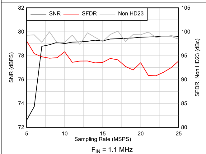
Figure 6-28. AC Performance vs Sampling Rate
