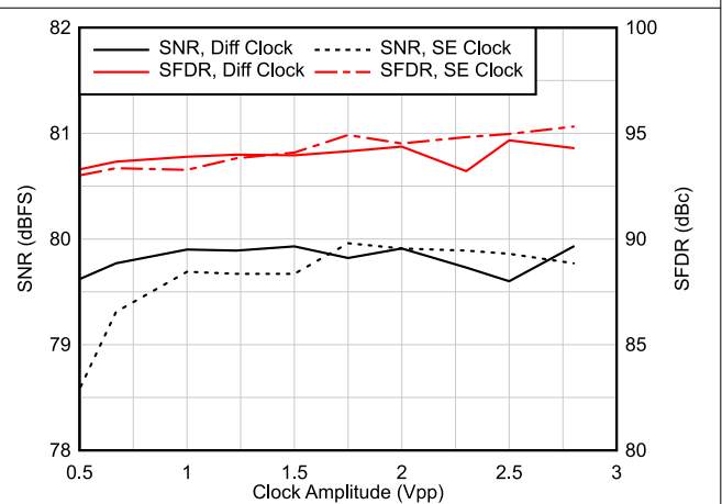
Differential (Diff) vs Single ended (SE) clock, F_{IN} = 5 MHz
