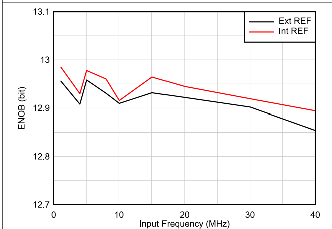
Figure 6-26. ENOB vs Input Frequency
