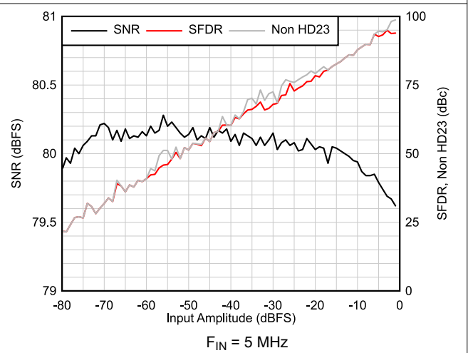
Figure 6-27. AC Performance vs Input Amplitude
