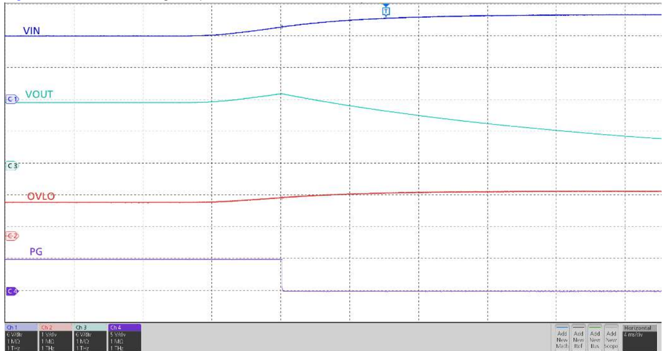
Figure 5-3. Overvoltage Protection Response of the TPS22811 Device
