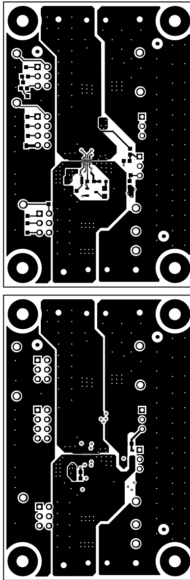
Figure 6-2. TPS22811EVM Board (a) Top Layer (b) Bottom Layer
