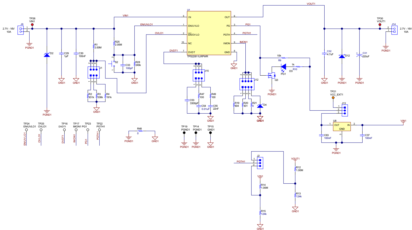
Figure 3-1. TPS22811EVM Load Switch Evaluation Board Schematic
