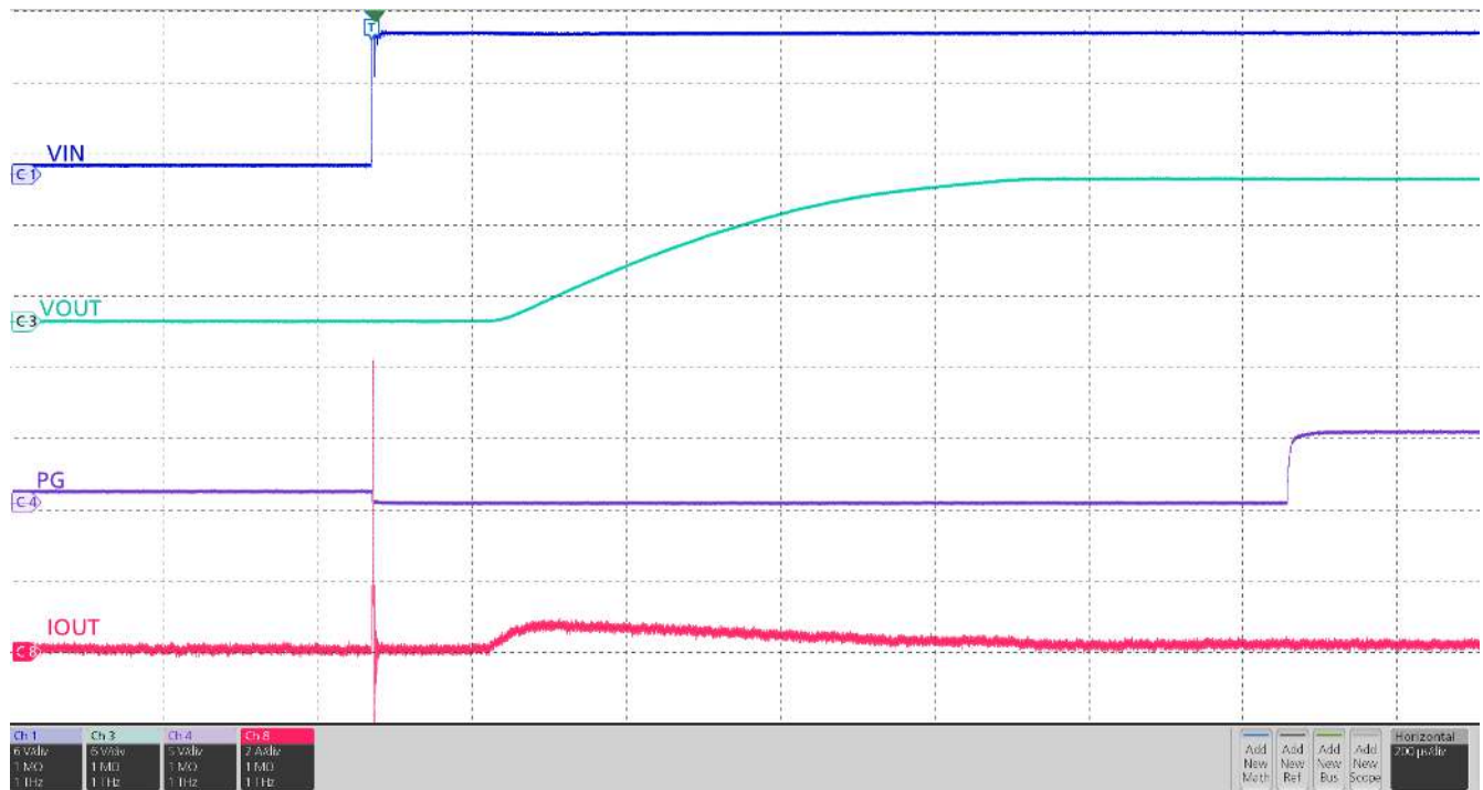
Figure 5-2. TPS22811 Output Rise Profile (VIN = 12 V, Cout = 10 \mu F, CdVdT = OPEN, No Load)
