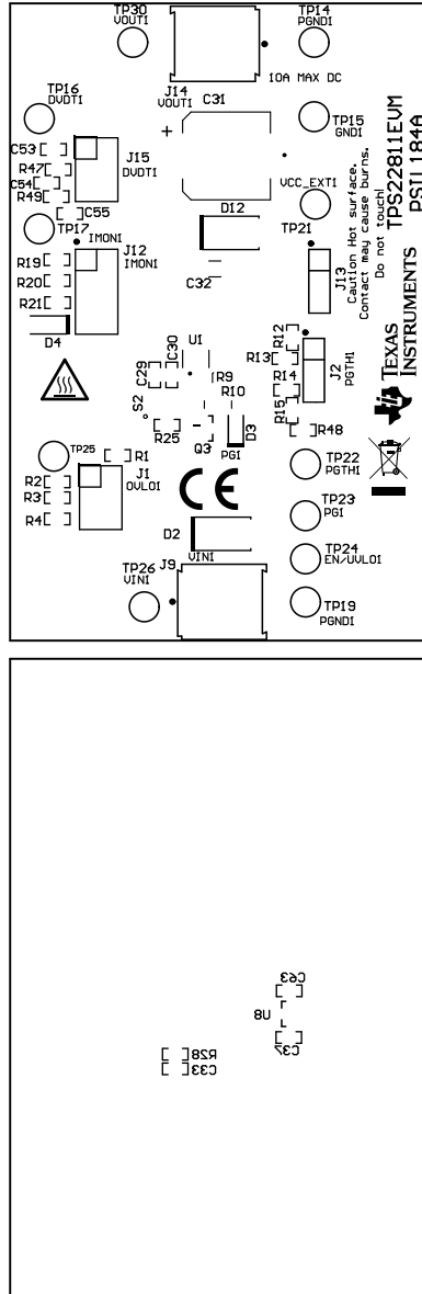
Figure 6-1. TPS22811EVM Board (a) Top Assembly (b) Bottom Assembly
