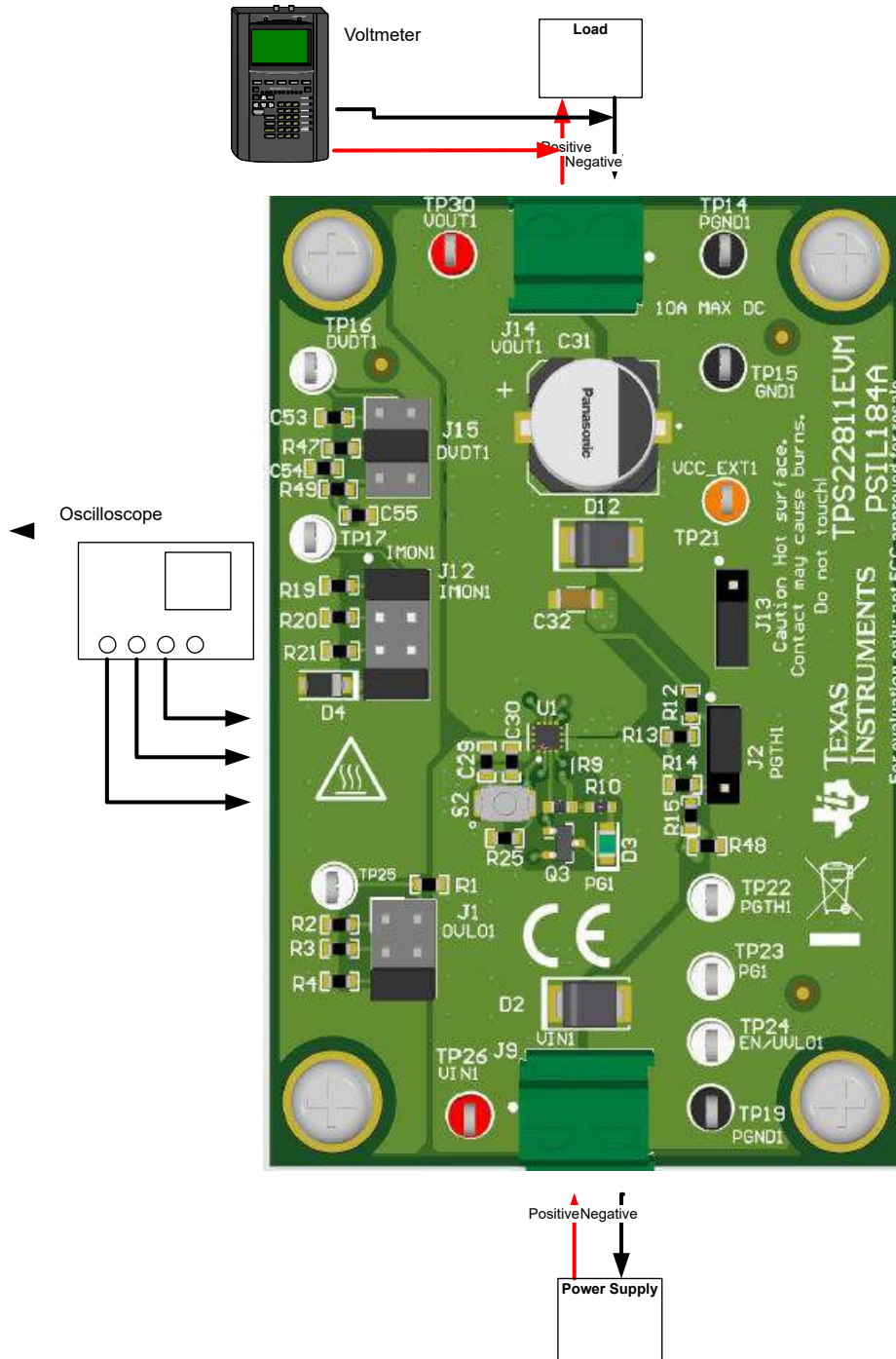
Figure 5-1. TPS22811EVM Setup with Test Equipment
