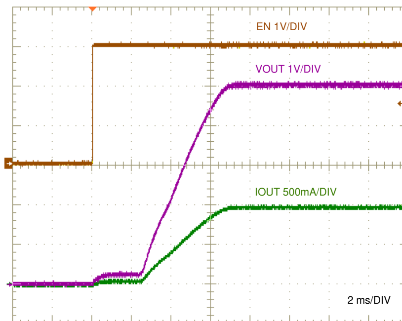
Figure 12. Enable On, V_{IN} = 24\text{ V} , I_{OUT} = 1\text{ A}
