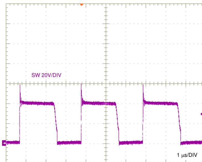
Figure 8. SW Node Voltage, V_{IN} = 24\text{ V} , I_{OUT} = 1\text{ A}
