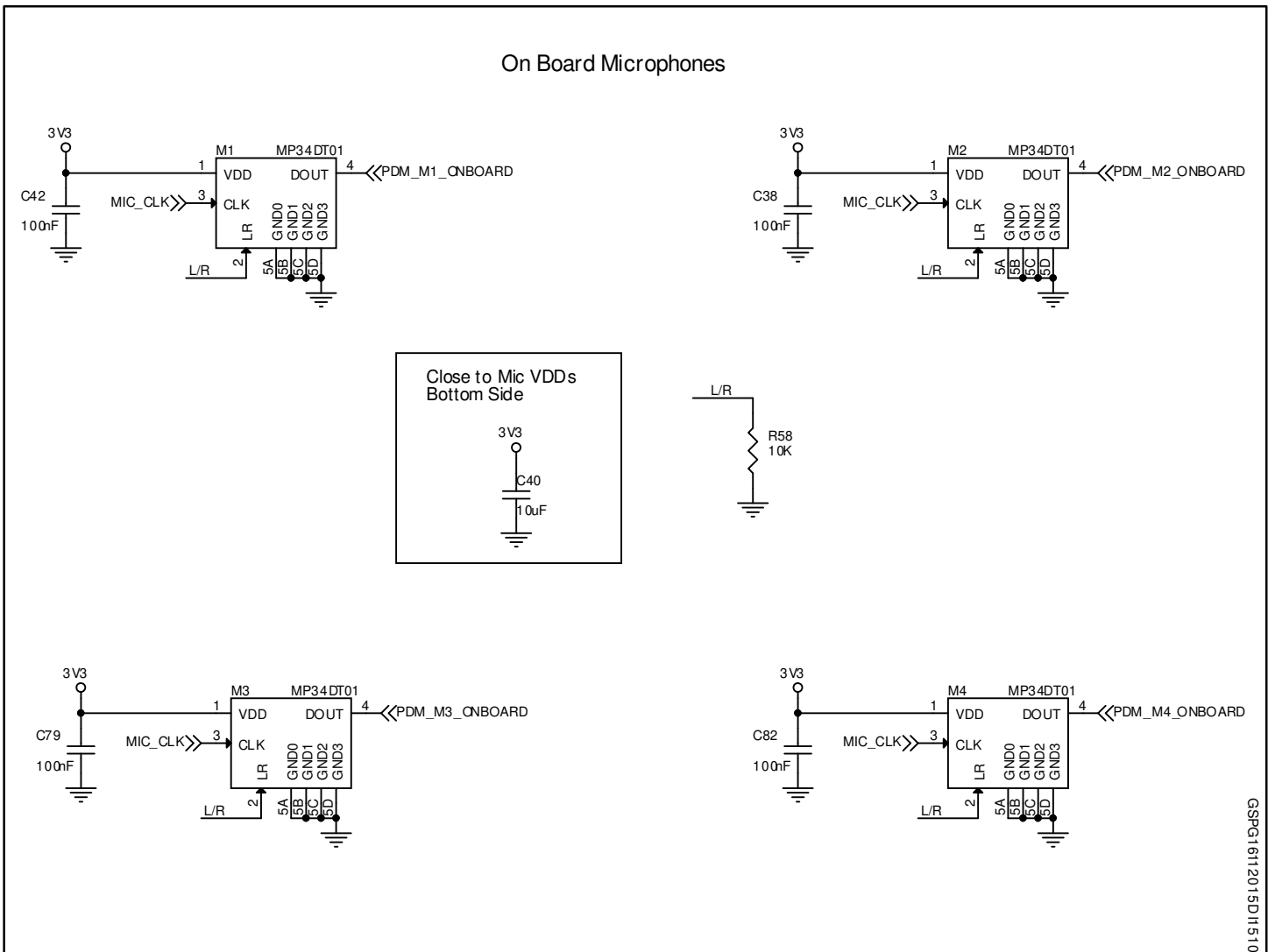
Figure 4: STEVAL-ID1001V1 board schematic part 4
