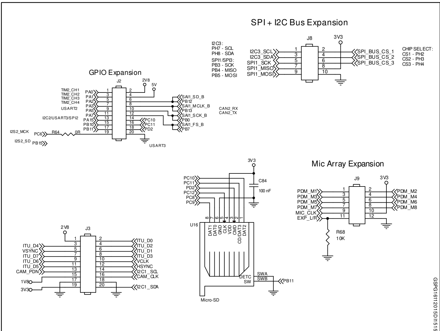
Figure 5: STEVAL-IDI001V1 board schematic part 5
