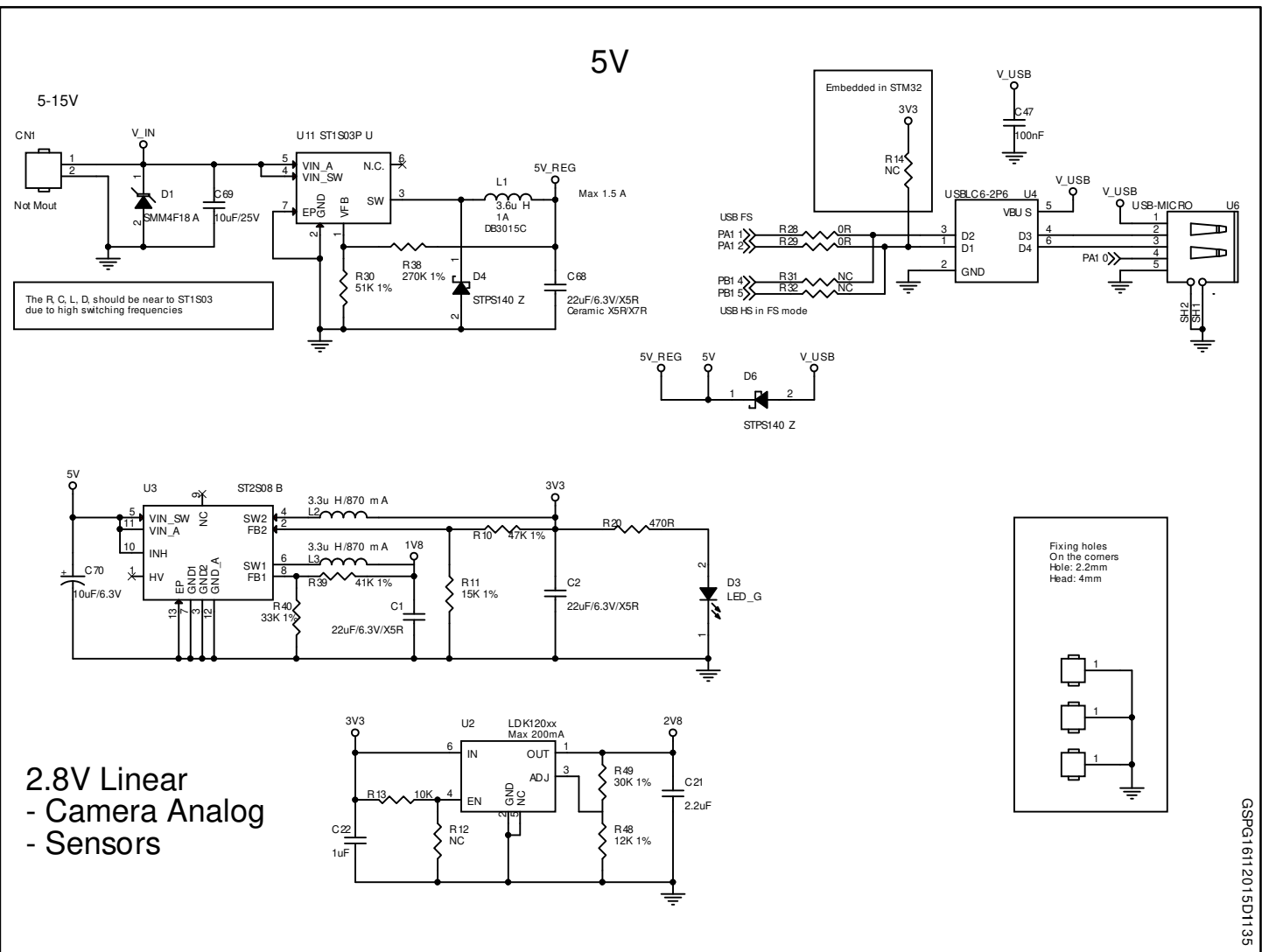
Figure 1: STEVAL-ID1001V1 board schematic part 1
