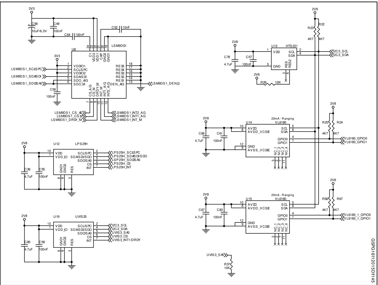
Figure 3: STEVAL-ID1001V1 board schematic part 3
