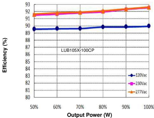
Figure 9: Efficiency vs. Output Power (Io=1.05A)
