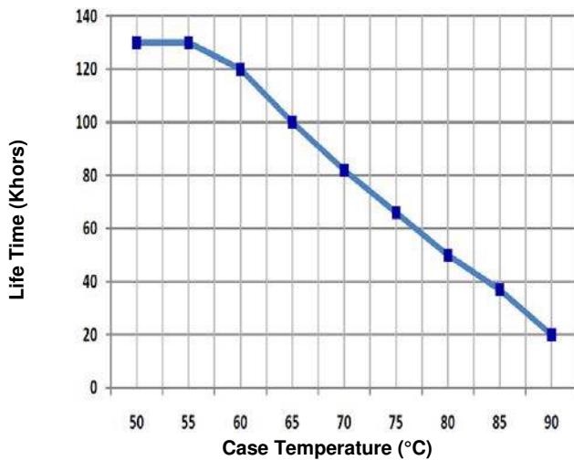
Figure 15: Life Time vs. Case Temperature
