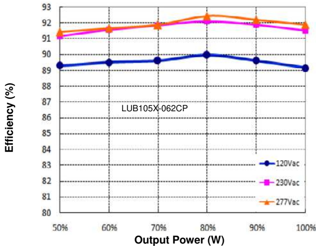
Figure 7: Efficiency vs. Output Power (Io=1.69A)
