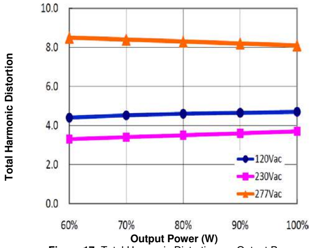
Figure 17: Total Harmonic Distortion vs. Output Power
