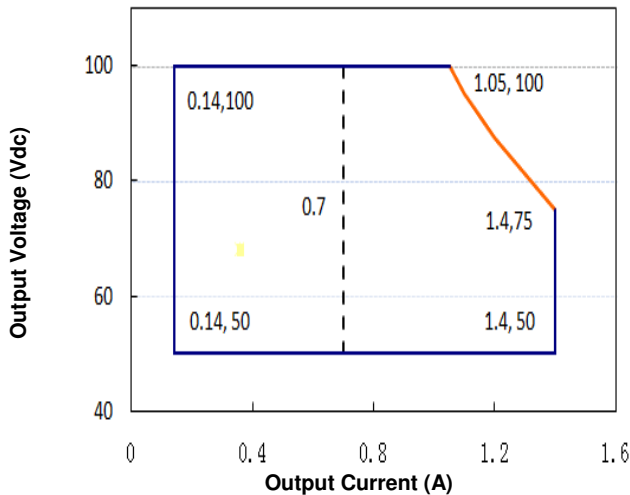
Figure 3: Typical V-I Characteristic Curve (LUB105X-100CP)
