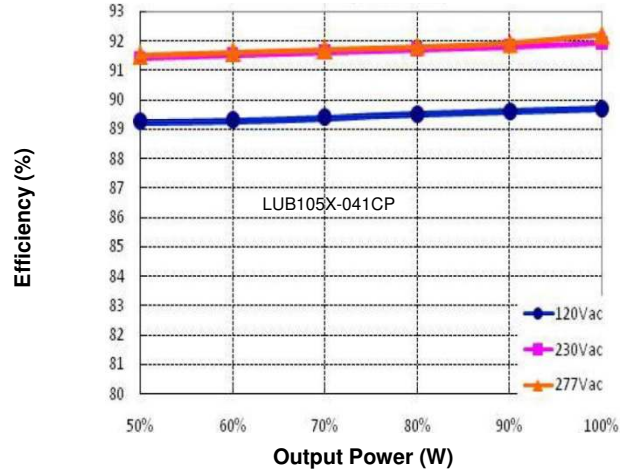
Figure 6: Efficiency vs. Output Power (Io=3.5A)
