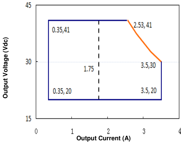
Figure 1: Typical V-I Characteristic Curve (LUB105X-041CP)
