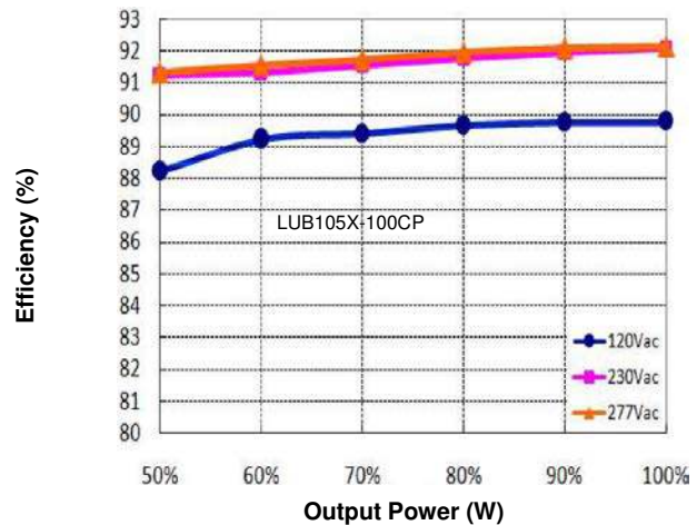
Figure 10: Efficiency vs. Output Power (Io=1.4A)
