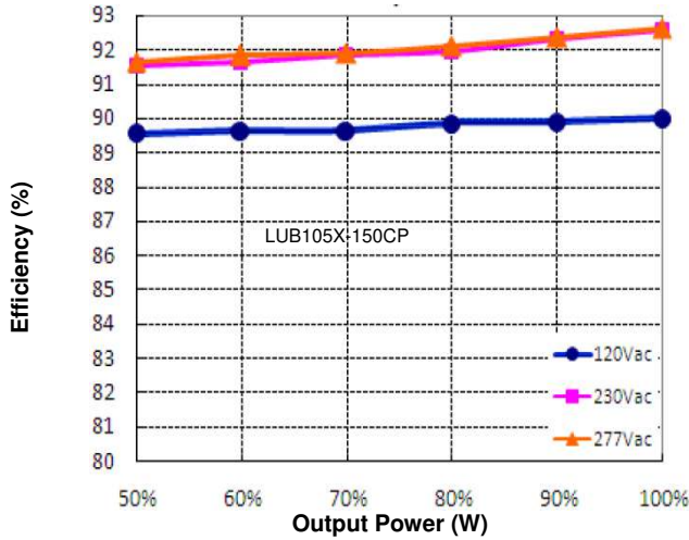
Figure 11: Efficiency vs. Output Power (Io=0.70A)
