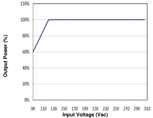
Figure 14: Output Power vs. Input Voltage
