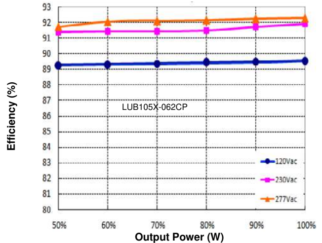
Figure 8: Efficiency vs. Output Power (Io=2.50A)
