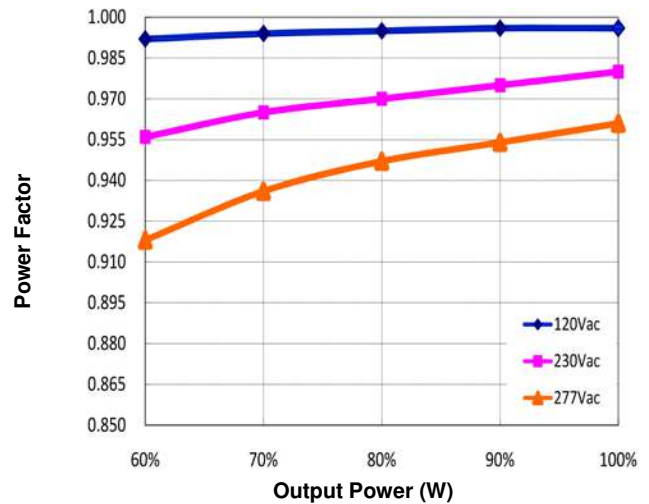
Figure 16: Power Factor vs. Output Power
