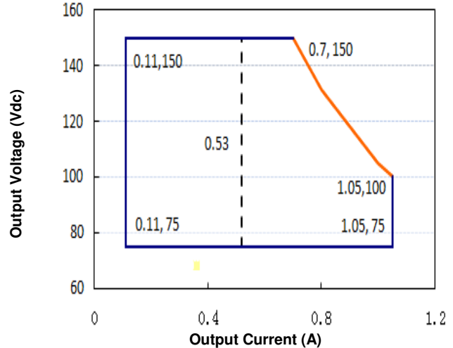
Figure 4: Typical V-I Characteristic Curve (LUB105X-150CP)
