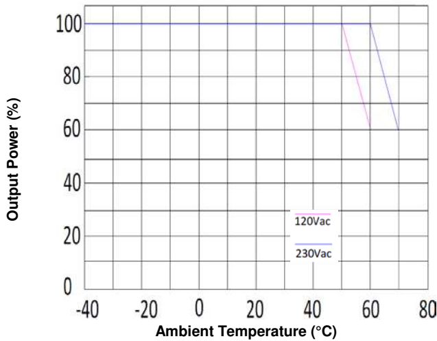
Figure 13: Output Power vs. Ambient Temperature
