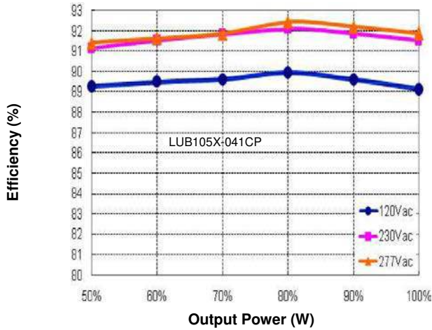
Figure 5: Efficiency vs. Output Power (Io=2.56A)
