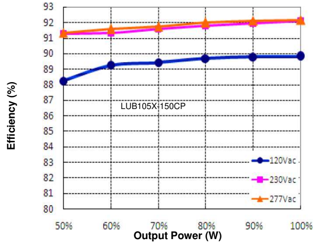
Figure 12: Efficiency vs. Output Power (Io=1.05A)
