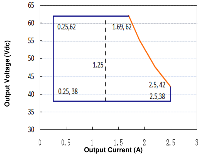
Figure 2: Typical V-I Characteristic Curve (LUB105X-062CP)
