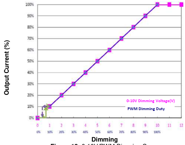
Figure 18: 0-10V/PWM Dimming Curve
