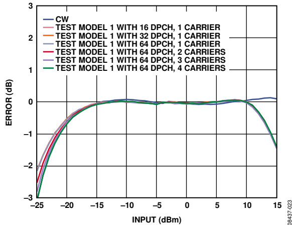
Figure 23. Error from CW Linear Reference vs. Input with Various W-CDMA Forward Link Waveforms at 2200 MHz, C_{FLTR} = 10 \text{ nF} , C_{OUT} = \text{Open}
