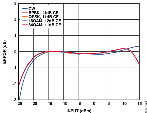
Figure 24. Error from CW Linear Reference vs. Input with Various 802.16 OFDM Waveforms at 3500 MHz, 10 MHz Signal BW, and 256 Subcarriers for All Modulated Signals, C_{FLTR} = 10 \text{ nF} , C_{OUT} = \text{Open}
