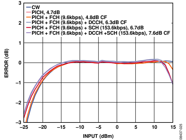
Figure 25. Error from CW Linear Reference vs. Input with Various CDMA2000 Reverse Link Waveforms at 1900 MHz, C_{FLTR} = 12 \text{ nF} , C_{OUT} = \text{Open}
