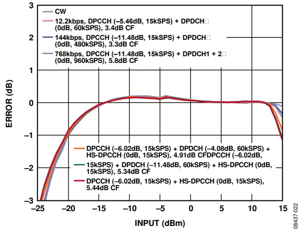
Figure 22. Error from CW Linear Reference vs. Input with Various W-CDMA Reverse Link Waveforms at 900 MHz, C_{FLTR} = 10 \text{ nF} , C_{OUT} = \text{Open}
