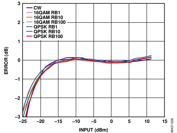
Figure 26. Error from CW Linear Reference vs. Input with Various LTE Reverse Link Waveforms at 2600 MHz, C_{FLTR} = 12 \text{ nF} , C_{OUT} = \text{Open}
