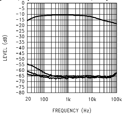
Figure 36. Top Trace = No Cap, Next Trace Down = 1µf Next Trace Down = 2µf, Bottom Trace = 4.7µf
