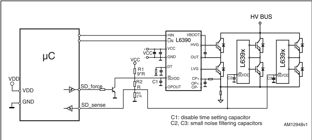
Figure 9. \overline{SD} level shifting example circuit
