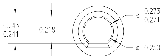
DETAIL A SCALE 2 : 1 (MOLDED HOLE)
