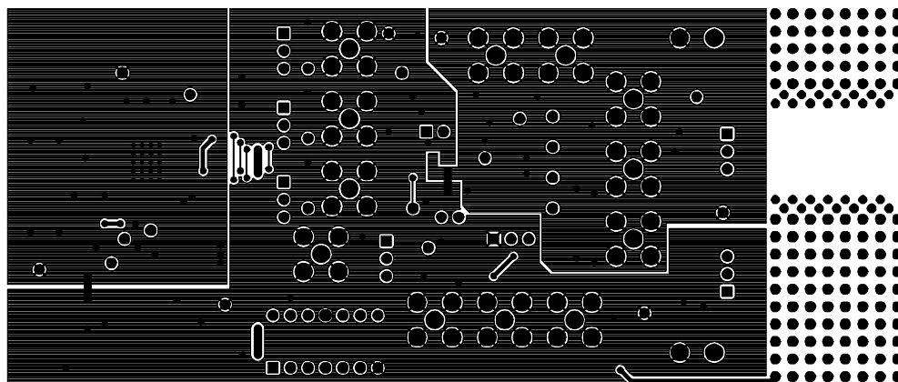
Eval-AD5930EB Rev. A – Component Side View
