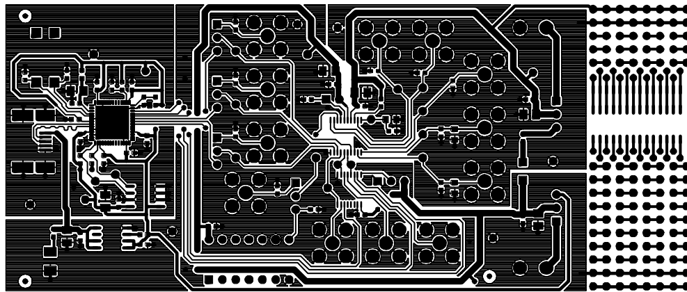
Eval-AD5930EB Rev. A – Component Side View Component Side
