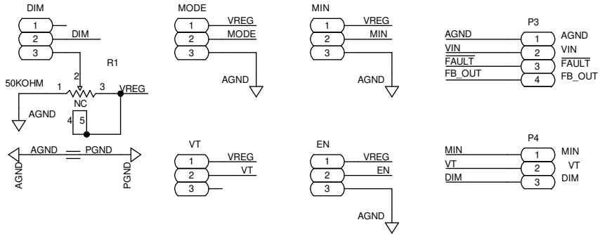
Figure 18. ADP8140EB-EVALZ Schematic Connectors and Peripherals
