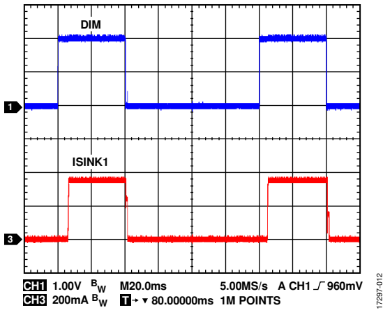
Figure 12. LED Current Pulsing with DIM
