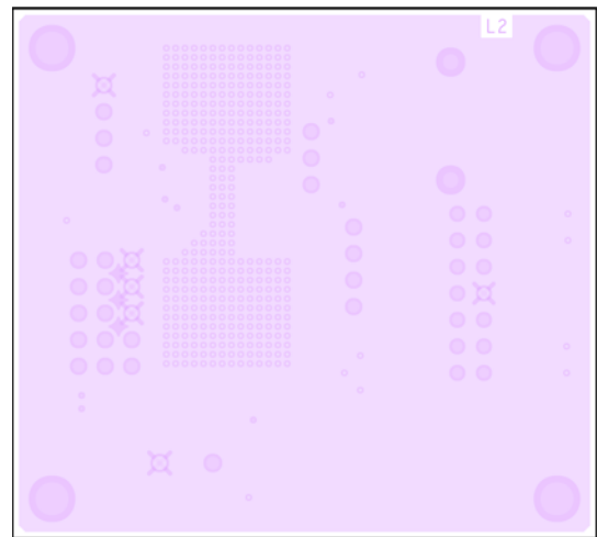
Figure 21. ADP8140EB-EVALZ Second Layer
