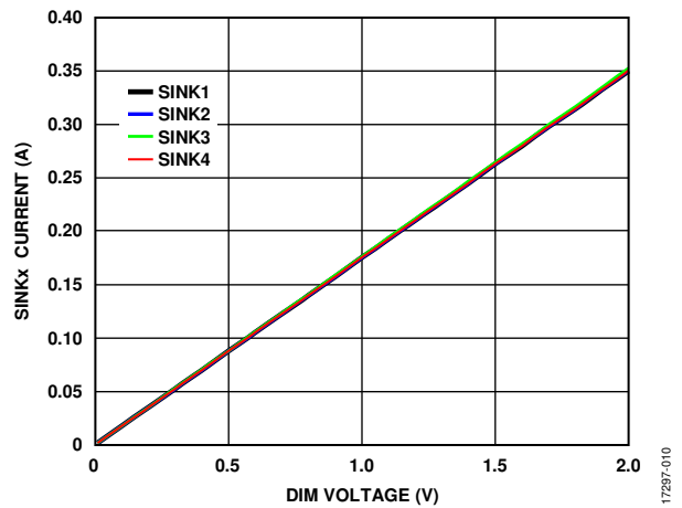
Figure 10. LED Current Scaling Using DC Voltage at DIM Pin
