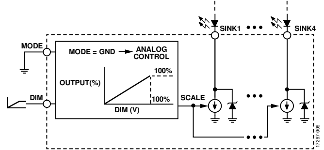
Figure 9. Reduced LED Current Using DC Voltage at DIM Pin
