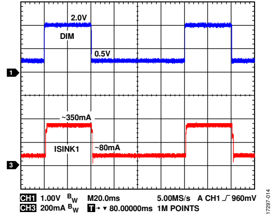
Figure 14. DIM Flexibility During LED Current Pulsing
