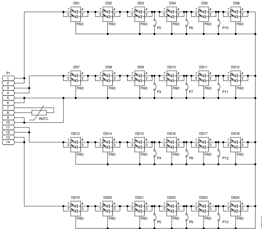
Figure 19. ADP8140 LED-EVALZ Schematic Connectors and Peripherals
