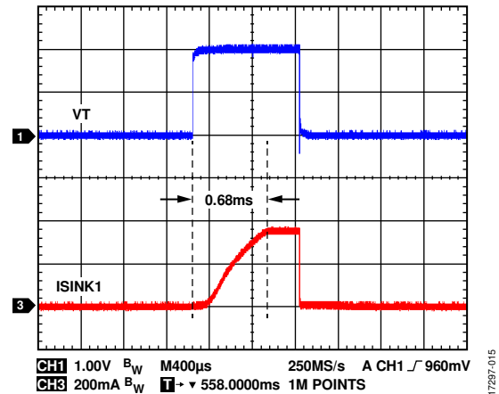
Figure 15. VT Speed During LED Current Pulsing
