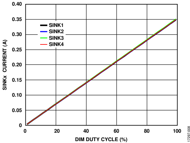
Figure 8. LED Current Scaling Using PWM Signal at DIM Pin
