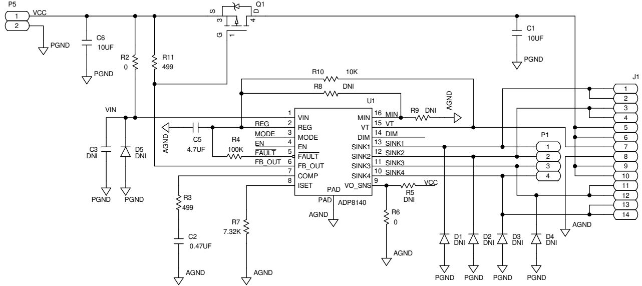
Figure 17. ADP8140EB-EVALZ Schematic
