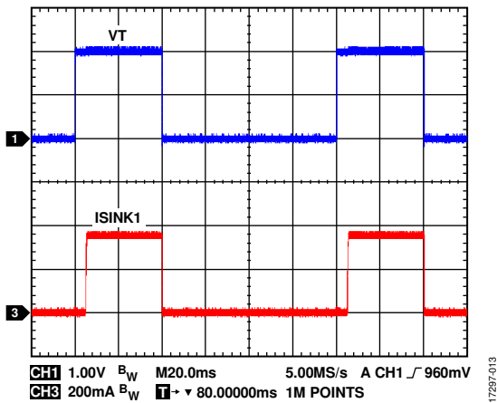
Figure 13. LED Current Pulsing with VT
