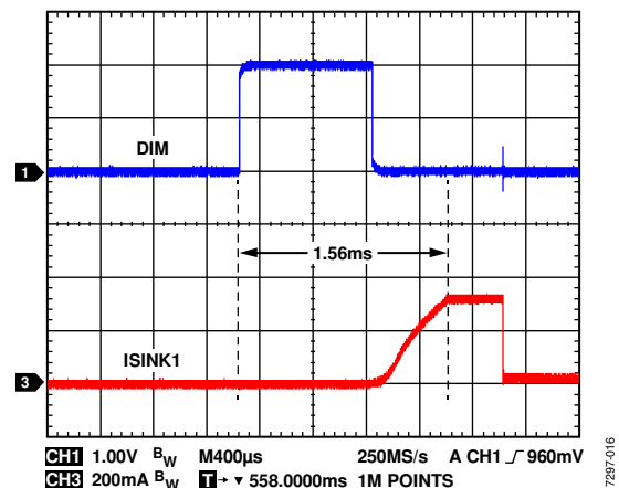
Figure 16. ISINK1 Response in 1 ms Pulse with DIM
