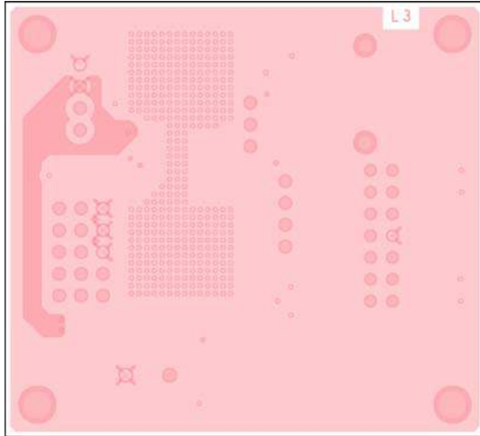
Figure 22. ADP8140EB-EVALZ Third Layer
