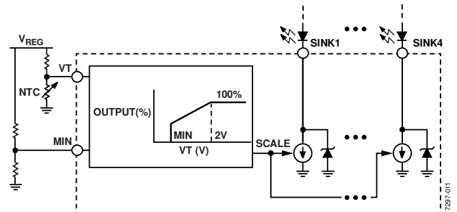
Figure 11. ADP8140 LED-EVALZ Board Current Scaling Using the VT Pin
