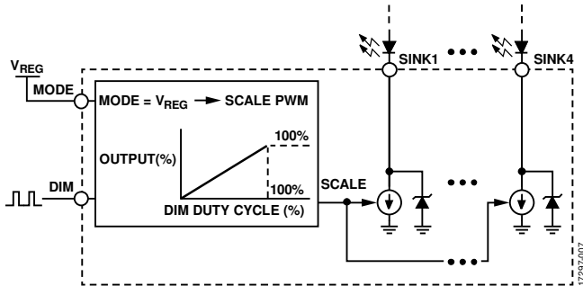
Figure 7. Reduced LED Current Using PWM Signal at DIM Pin
