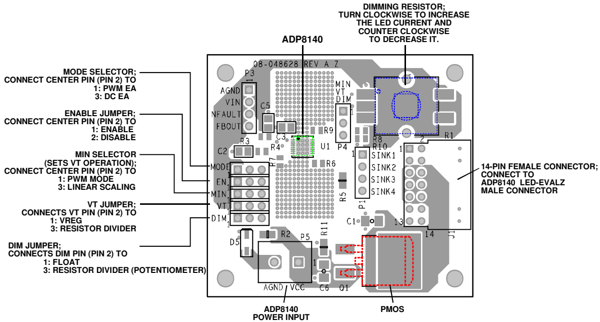
Figure 2. ADP8140EB-EVALZ Features
