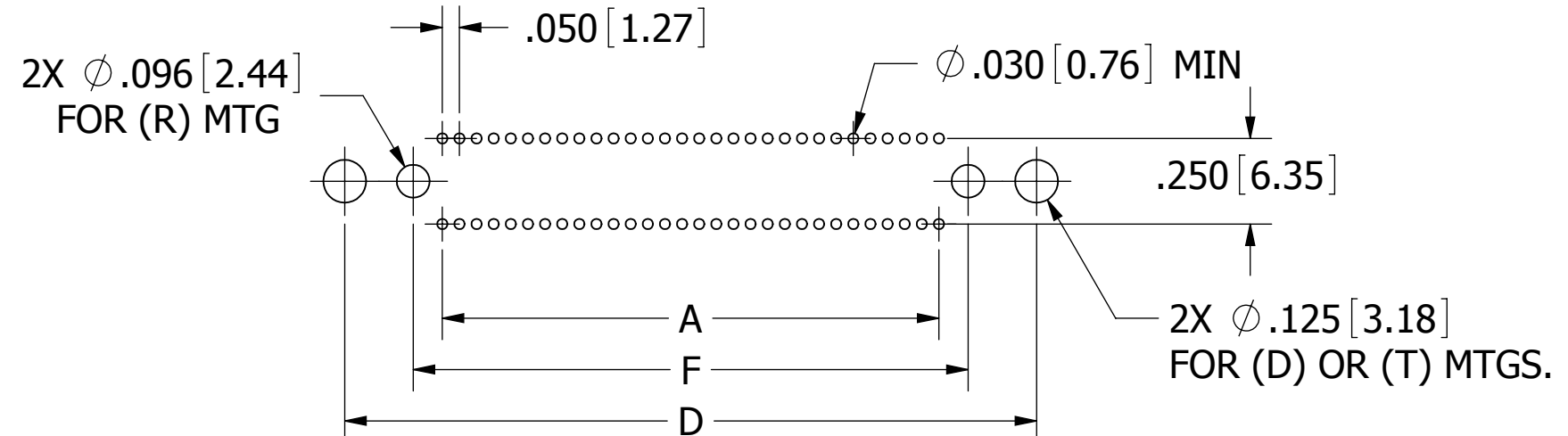
PCB LAYOUT, CONNECTOR SIDE
