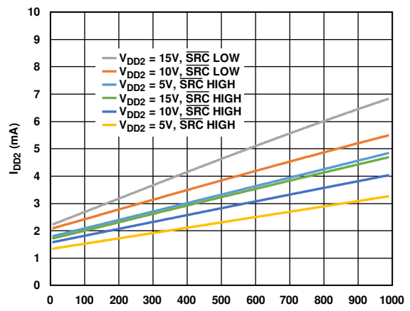
Figure 15. I_{DD2} vs. Frequency, 50% Duty Cycle, No Load
