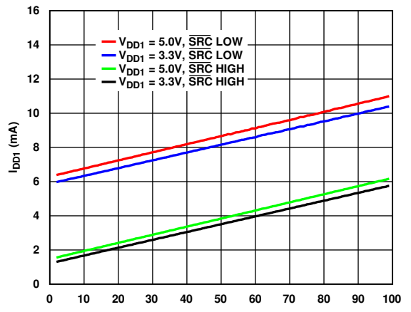
Figure 14. I_{DD1} vs. Duty Cycle, 10 kHz Input Signal
