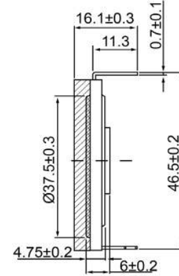
SIDE VIEW (2)
