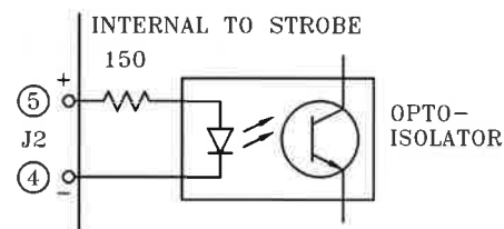
Figure 3: Input Trigger Circuit
