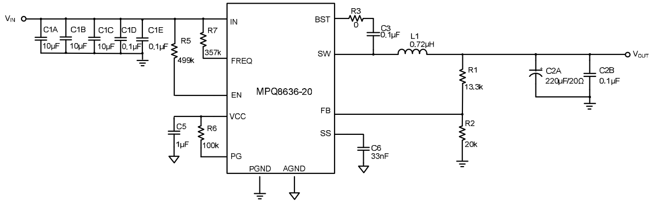
Figure 10 — Typical Application Circuit with No External Ramp MPQ8636-20, V_{IN}=12V , V_{OUT}=1V , I_{OUT}=20A , f_{SW}=500kHz
