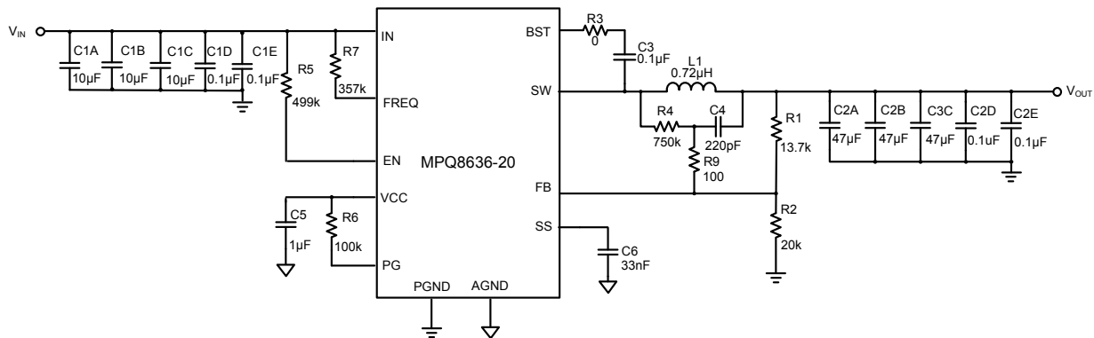
Figure 11 — Typical Application Circuit with Low ESR Ceramic Capacitor MPQ8636-20, V_{IN}=12V , V_{OUT}=1V , I_{OUT}=20A , f_{SW}=500kHz
